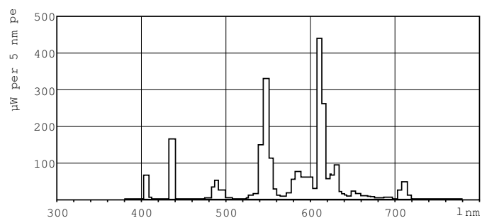
LDPB_PLS2PLM_827-Spectral power distribution B/W
