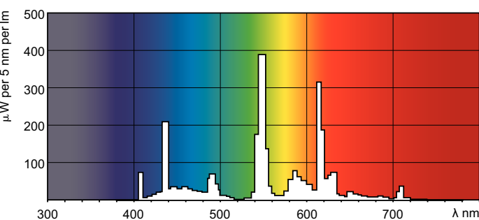
LDPO_PLS4PLM_840-Spectral power distribution Colour
