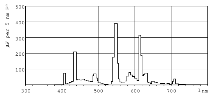
LDPB_PLS4PLM_840-Spectral power distribution B/W
