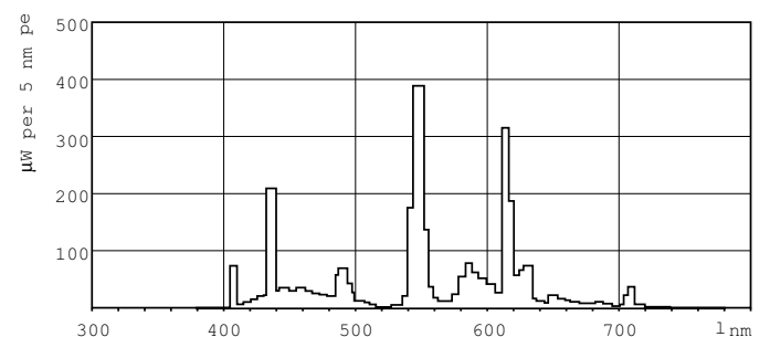
LDPB_PLC2P_840-Spectral power distribution B/W
