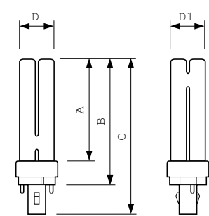
PL-C 18W/865/2P
