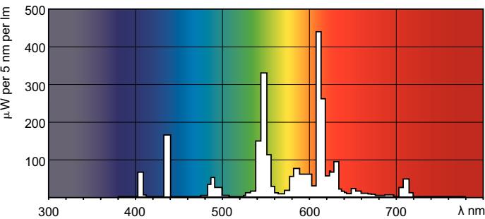
LDPO_PLT4PN_827-Spectral power distribution Colour
