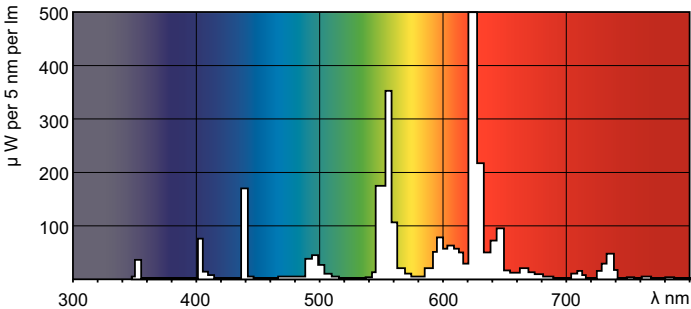
LDPO_TL5-HE8_827-Spectral power distribution Colour
