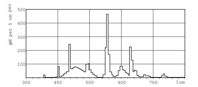
LDPB_TL5-HO8_865-Spectral power distribution B/W
