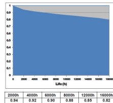
LUMEN MAINTENANCE
