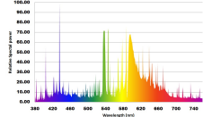
Spectral Power Distribution Relumina lamps
