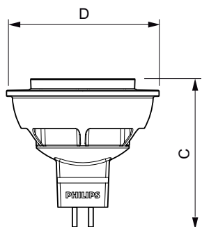
LED VLE D 6.3-35W 840 MR16 36D
