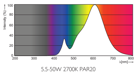
5.5-50W 2700K PAR20
