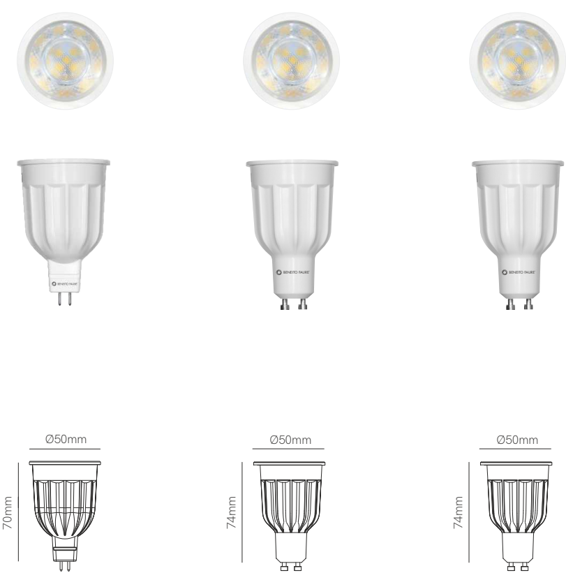
Power MR16
