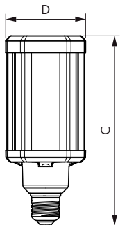
Tforce LED HPL ND 3klm E27 840 CL IP65
