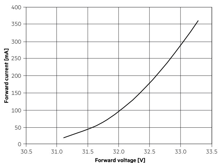
SLE 06mm 1600lm ADV8
