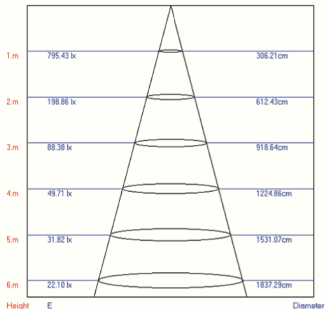
Lux-Distance Curve
