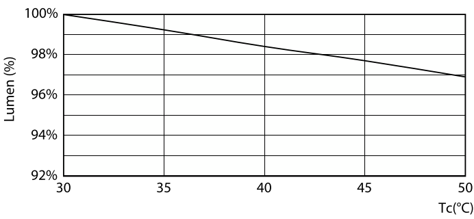
Lumen Maintenance Diagram - LED 4.5W 310mm S19 WW ND 1CT/4
