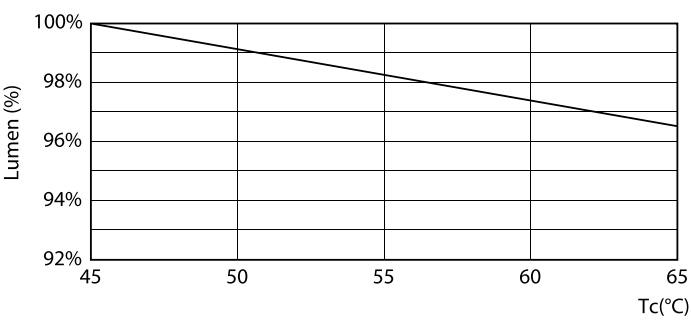
Lumen Maintenance Diagram - CorePro LED PLS 3.5W 840 2P G23
