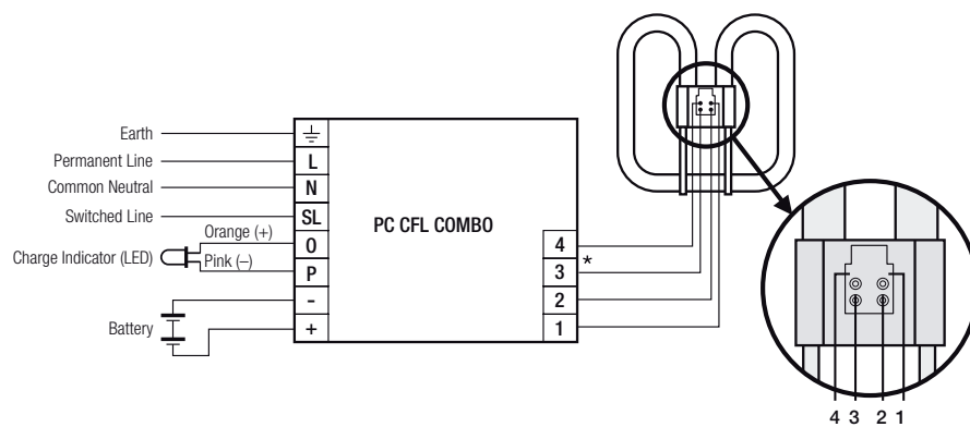
Circuit diagram PC CFL COMBO with single TC-DD lamp
