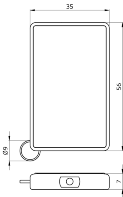
Dimensions 92159
