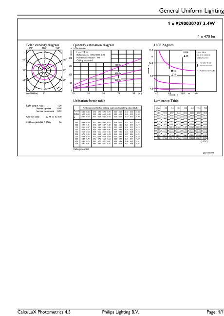
General uniform lighting - MAS VLE LEDBulbD3.4-40W E27 927 A60 FR G
