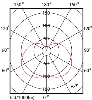
Light Distribution Diagram - CorePro LED Stick ND 9.5-75W T38 E27 840
