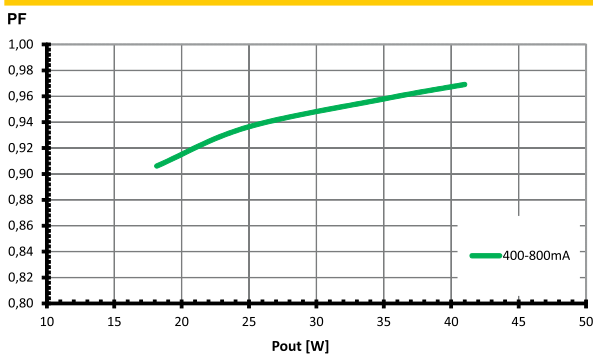
Power factor
