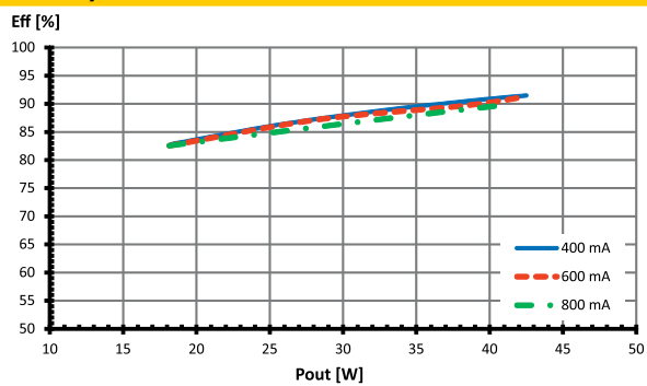
Efficiency
