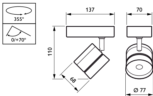
CoreLine Projector ST120C/ST120T
